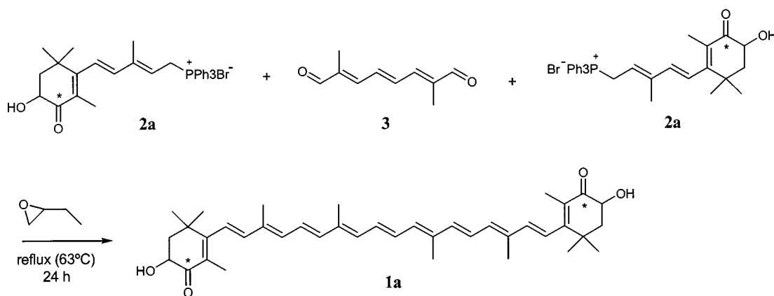
Scheme 2. Synthesis of (4,4'- ^{13}\text{C}_2 )astaxanthin ( 1a ) from (4- ^{13}\text{C} )phosphonium salt ( 2a ); labelled positions are marked with an asterisk
