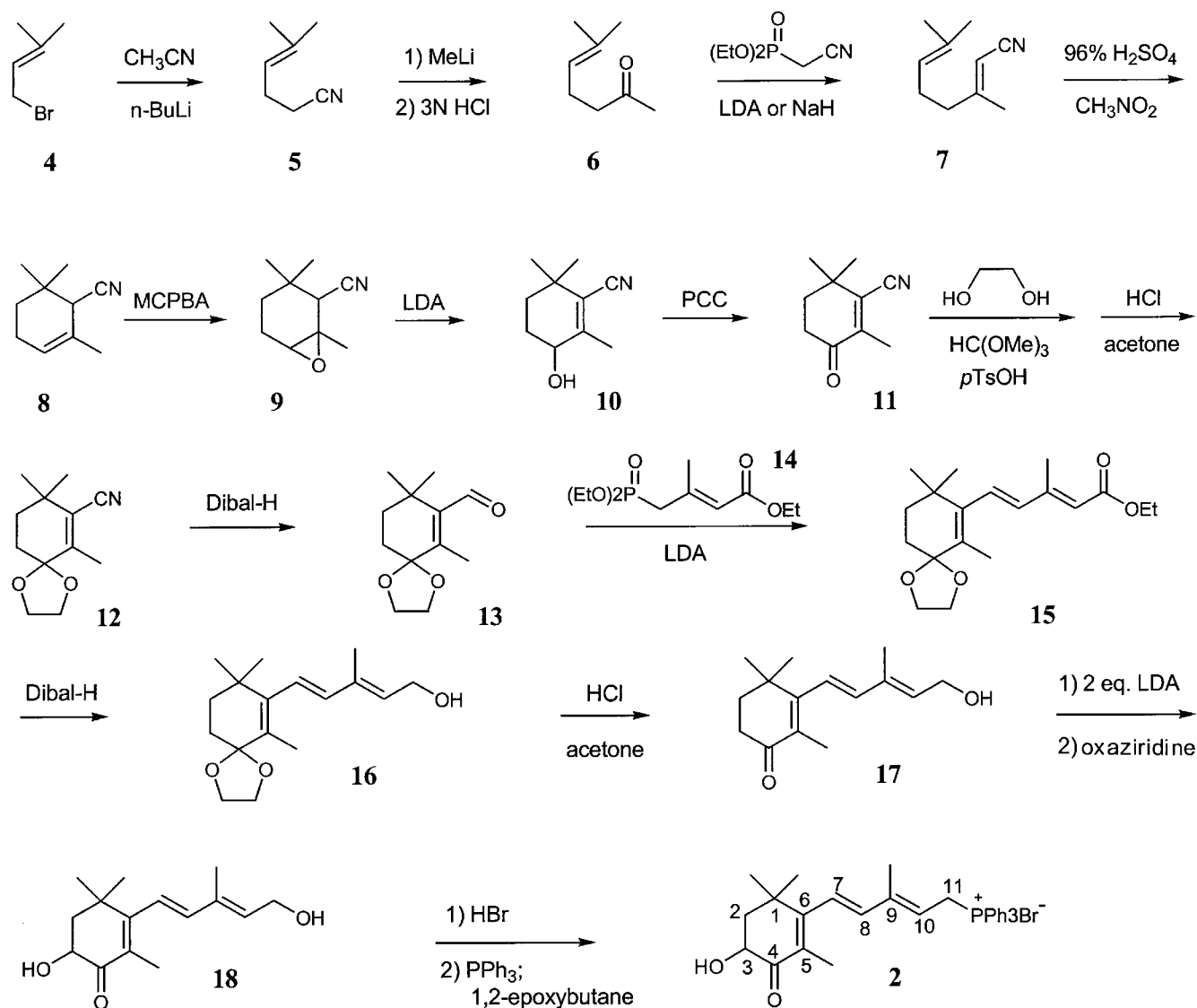
Scheme 1. Synthesis of the C 15 -phosphonium salt 2 ; when (2- 13 C)acetonitrile is used as starting material, (4- 13 C)phosphonium salt 2a is obtained
